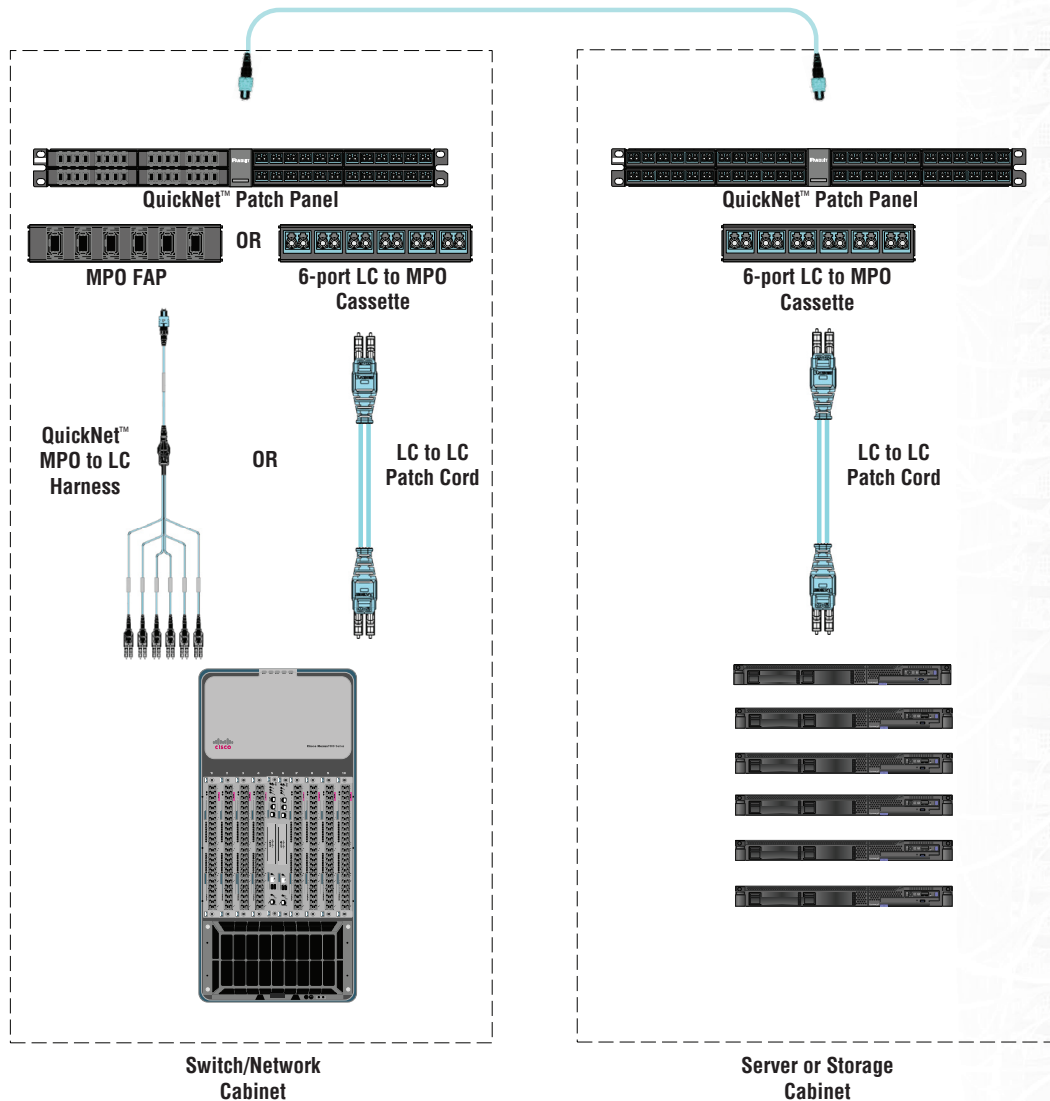
Figure 2 – Two-Connector Channel
