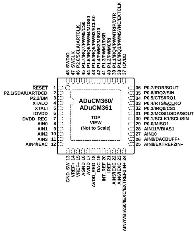
Figure 8. Pin Configuration
