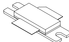
CASE 465-06, STYLE 1 NI-780 MRF9080
