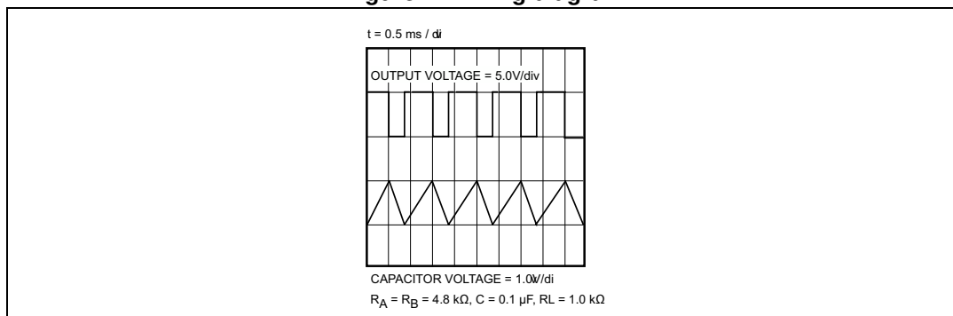
Figure 7. Timing diagram
