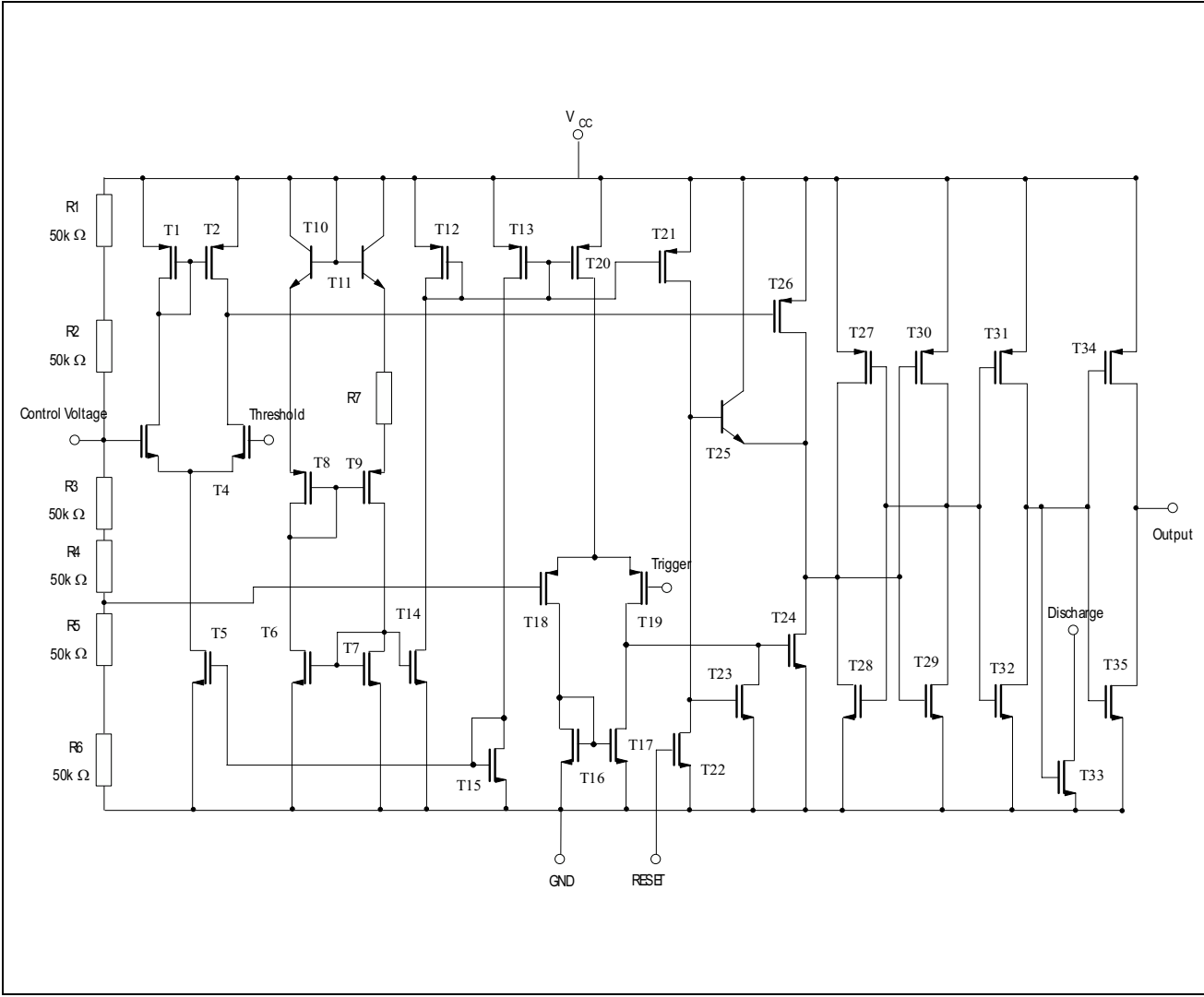
Figure 1. Schematic diagram
