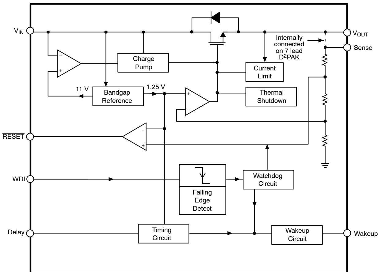
Figure 2. Block Diagram
