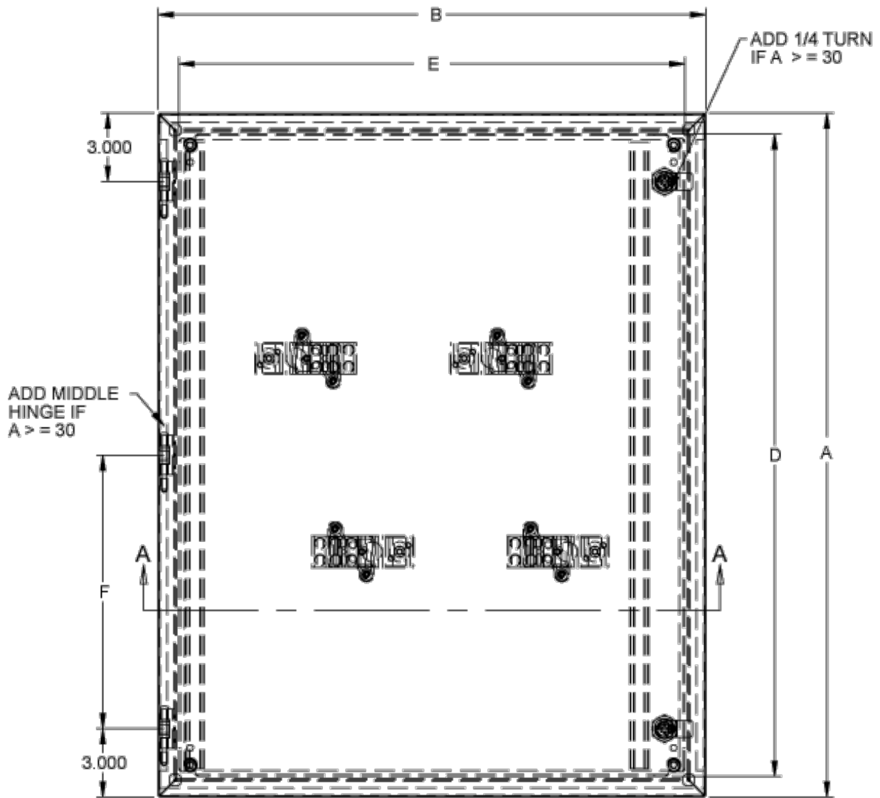
Front View
