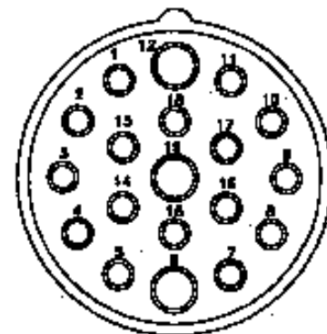
Femelle - Female - Buchse
