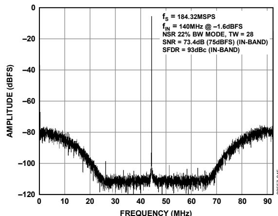
Figure 46. 22% BW Mode, Tuning Word = 28 ( f_s/4 Tuning)
