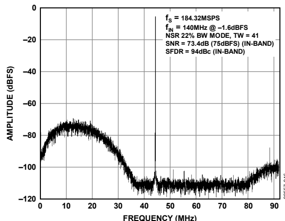
Figure 47. 22% BW Mode, Tuning Word = 41
