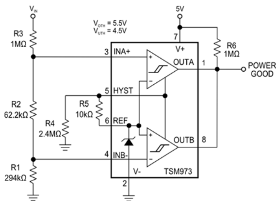
Figure 4. Window Detector
