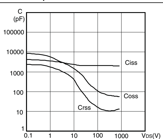
Figure 13. Capacitance variations
