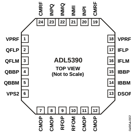
Figure 2. LFCSP Pin Configuration
