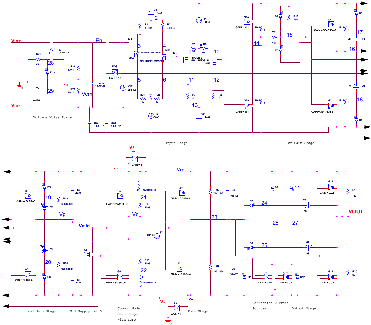
FIGURE 21. SPICE SCHEMATIC
