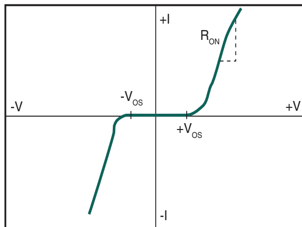
3.3 Figure 3: Switch 4
