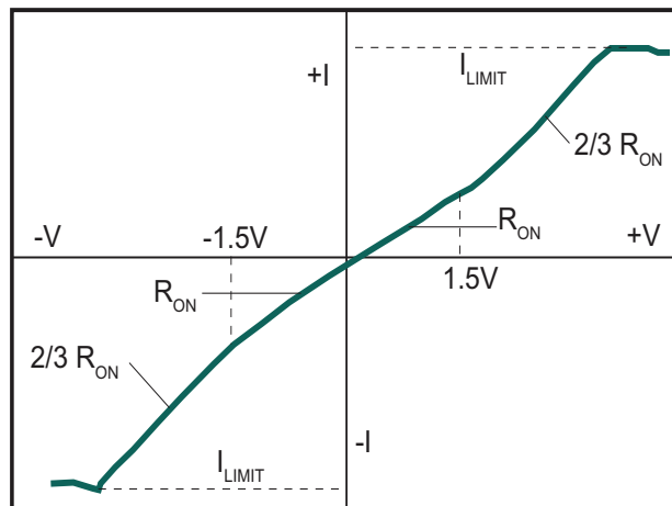
3.4 Figure 4: Switches 5-6
