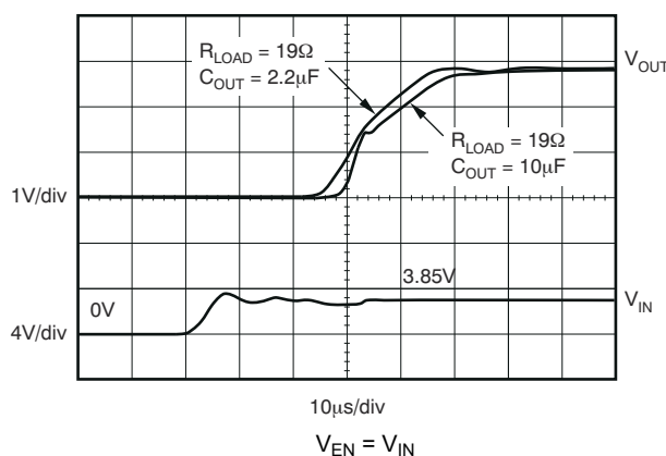
Figure 6-23. TPS799285 Turn-On Response
