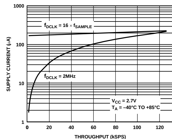
Figure 35. Supply Current vs. Throughput (μA)
