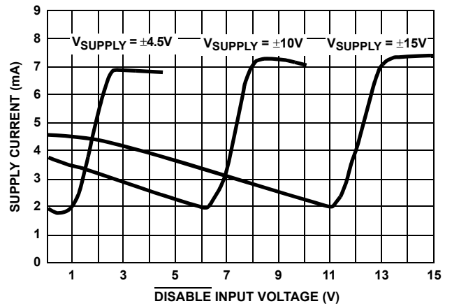
FIGURE 16. SUPPLY CURRENT vs \overline{\text{DISABLE}} INPUT VOLTAGE
