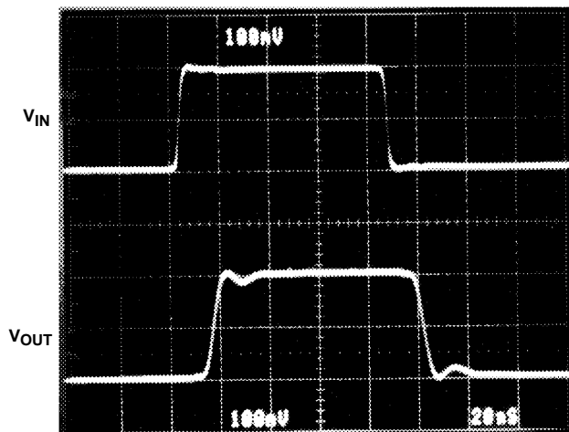
FIGURE 4. SMALL SIGNAL RESPONSE
