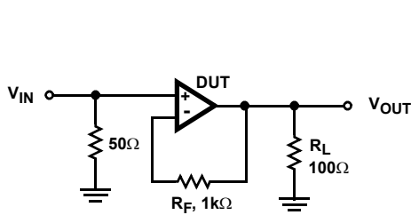
FIGURE 2. SMALL SIGNAL PULSE RESPONSE CIRCUIT
