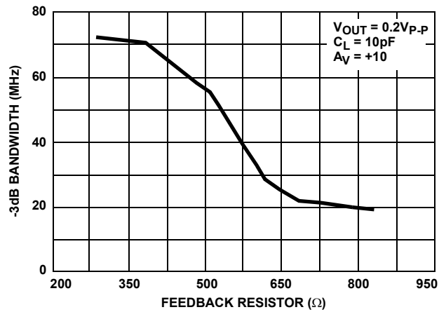
FIGURE 45. BANDWIDTH vs FEEDBACK RESISTANCE
