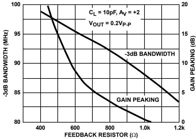
FIGURE 25. BANDWIDTH AND GAIN PEAKING vs FEEDBACK RESISTANCE
