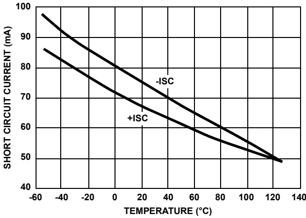
FIGURE 31. SHORT CIRCUIT CURRENT LIMIT vs TEMPERATURE
