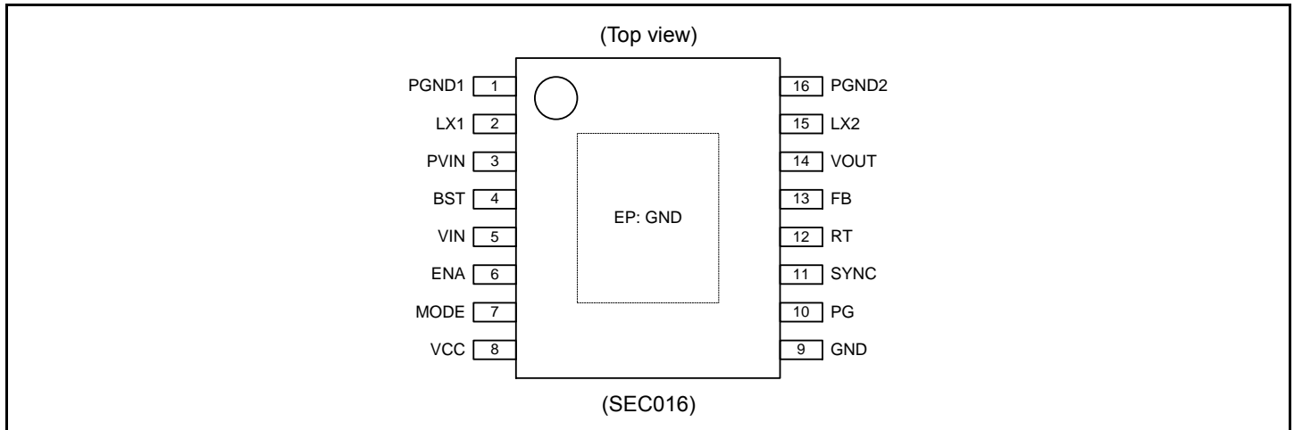
Figure 1-1 Pin Assignment
