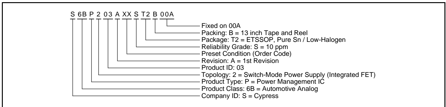
Figure 13-1 Ordering Part Number Definitions
