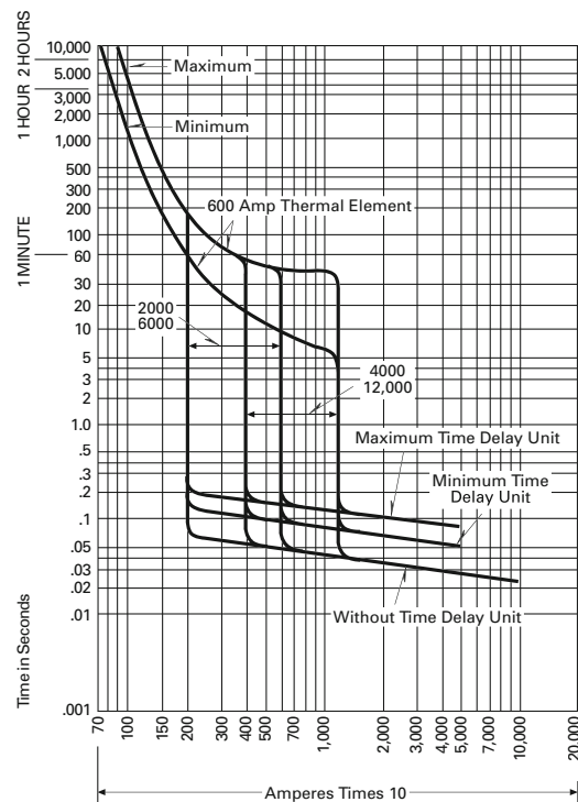
EXPANDED TIME DELAY CURVE
