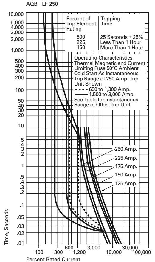
AQB-LF250 BREAKERS
