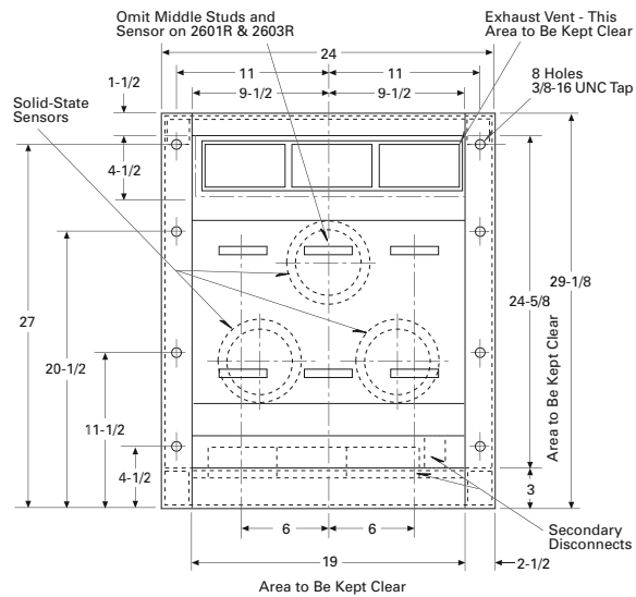
REAR VIEW
