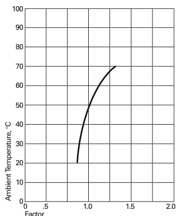
DERATING CURVE
