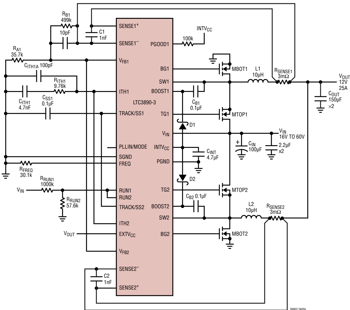
High Efficiency 12V at 25A Dual-Phase Step-Down Converter
