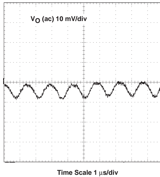
Figure 2-19. Measured Output Voltage Ripple, TPS54872
