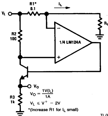
Current Monitor
