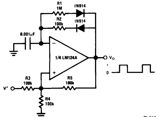
Pulse Generator
