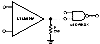
Driving TTL
