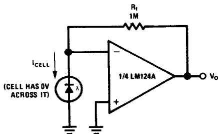
Photo Voltaic-Cell Amplifier
