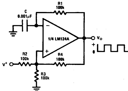
Squarewave Oscillator
