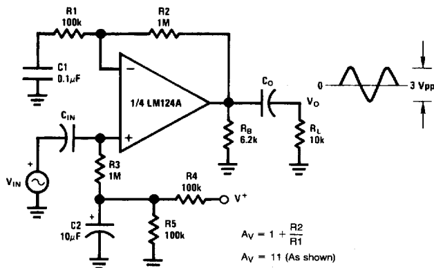
AC Coupled Non-Inverting Amplifier
