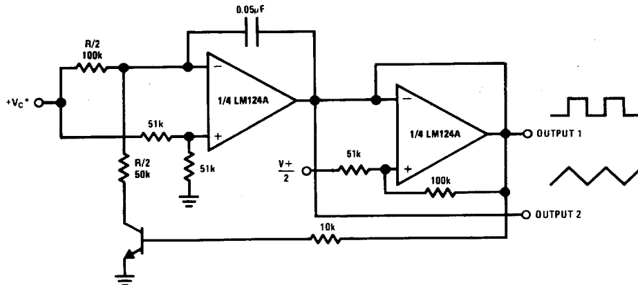
Voltage Controlled Oscillator Circuit
