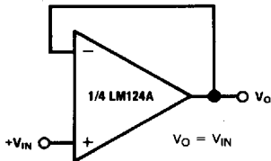
Voltage Follower
