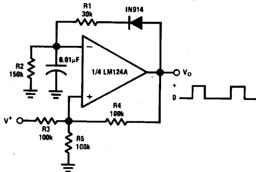
Pulse Generator
