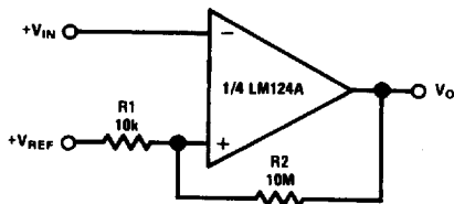
Comparator with Hysteresis
