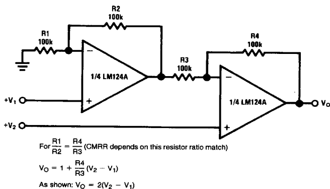
High Input Z, DC Differential Amplifier
