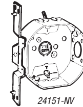
24151-NV V bracket recessed 1/4"
