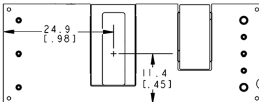
Figure 17. Pick and Place Location.
