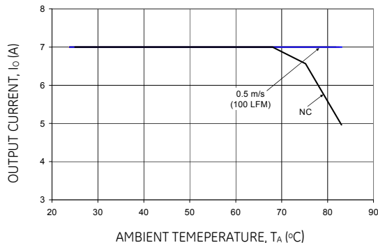
Figure 18. Output Current Derating for the Module with Heatplate and 1.0 in. heat sink; Airflow in the Transverse Direction from Vout(+) to Vout(-); Vin = 48V.
