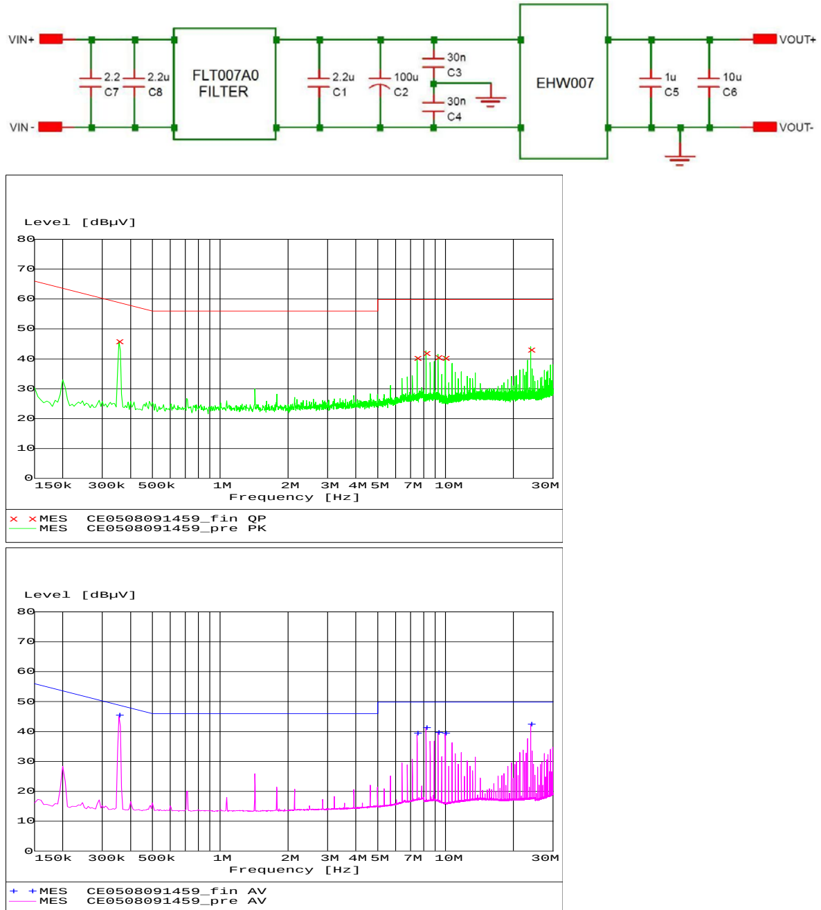
Figure 21. EMC Considerations
