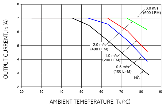
Figure 14. Output Current Derating for the Open Frame Module; Airflow in the Transverse Direction from Vout(+) to Vout(-); V_{in} = 48V .
