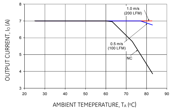
Figure 17. Output Current Derating for the Module with Heatplate and 0.5 in. heat sink; Airflow in the Transverse Direction from Vout(+) to Vout(-); V_{in} = 48V .
