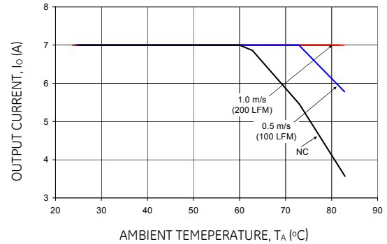
Figure 16. Output Current Derating for the Module with Heatplate and 0.25 in. heat sink; Airflow in the Transverse Direction from Vout(+) to Vout(-); V_{in} = 48V .
