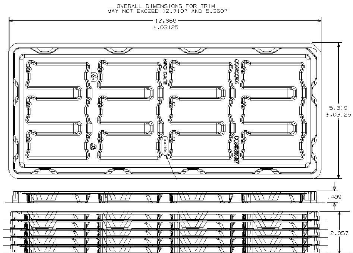
Figure 22. Surface Mount Packaging Tray
