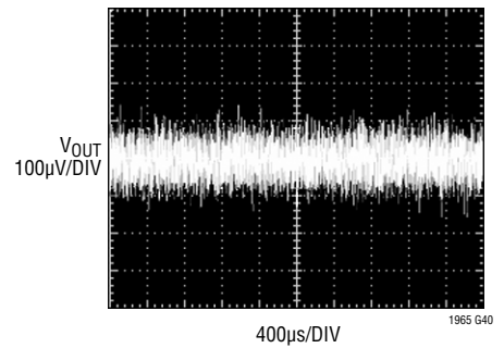
LT1965-1.8 10Hz to 100kHz Output Noise
