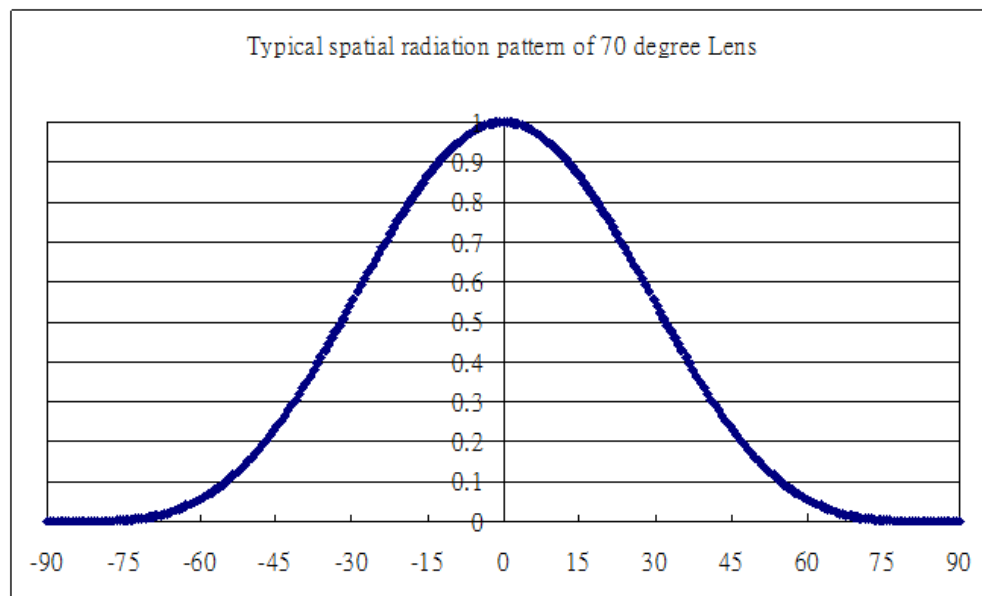
Fig. (70° Lens) Typical Representative Spatial Radiation Pattern
