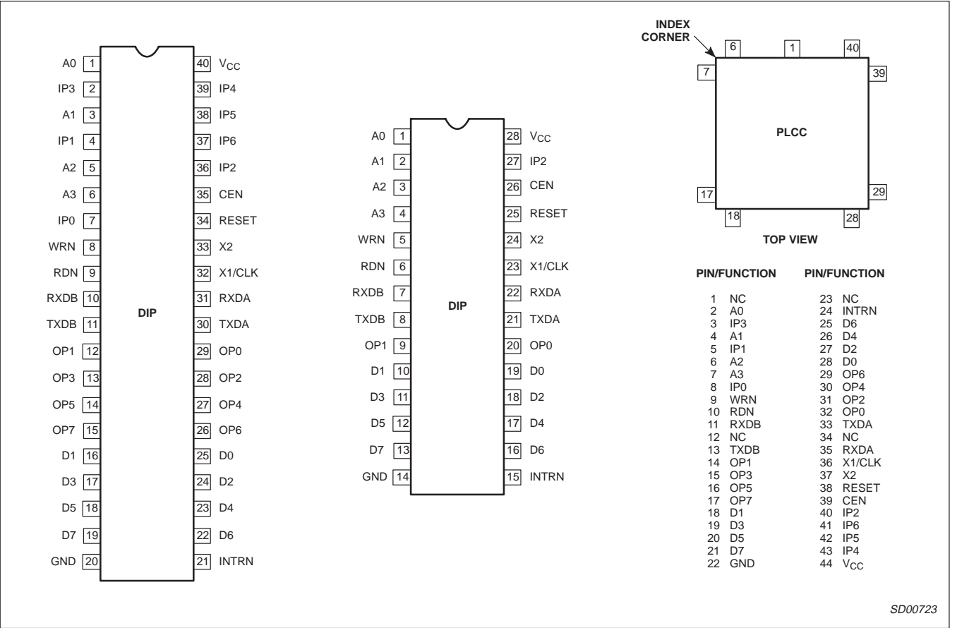
Figure 1. Pin configurations
