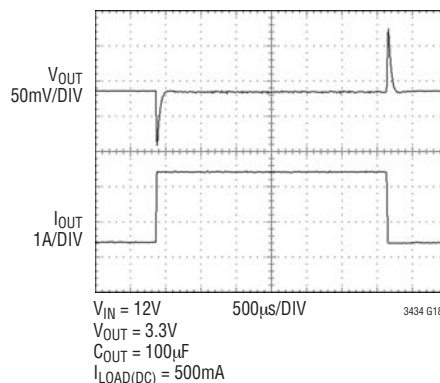
Step Response
