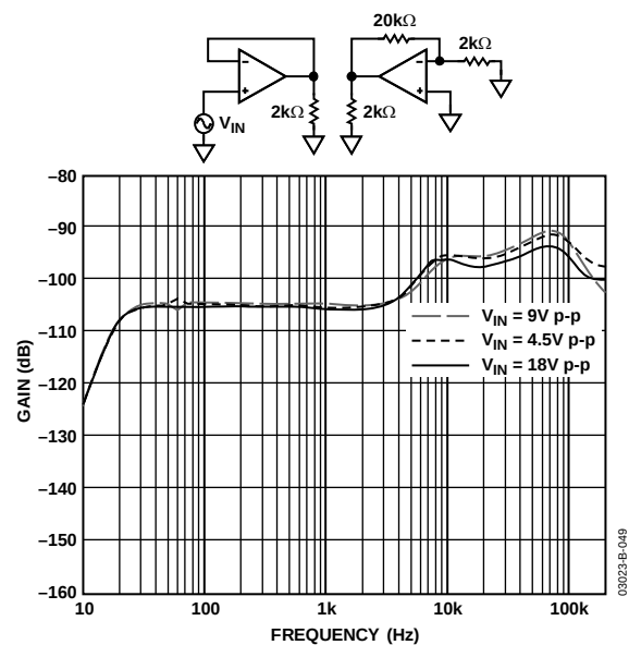
Figure 38. Channel Separation
