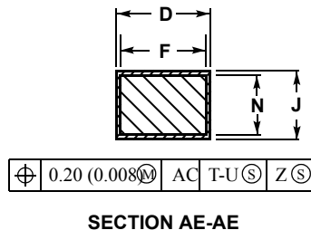
Figure 5-2 100-pin LQPF Mechanical Information
