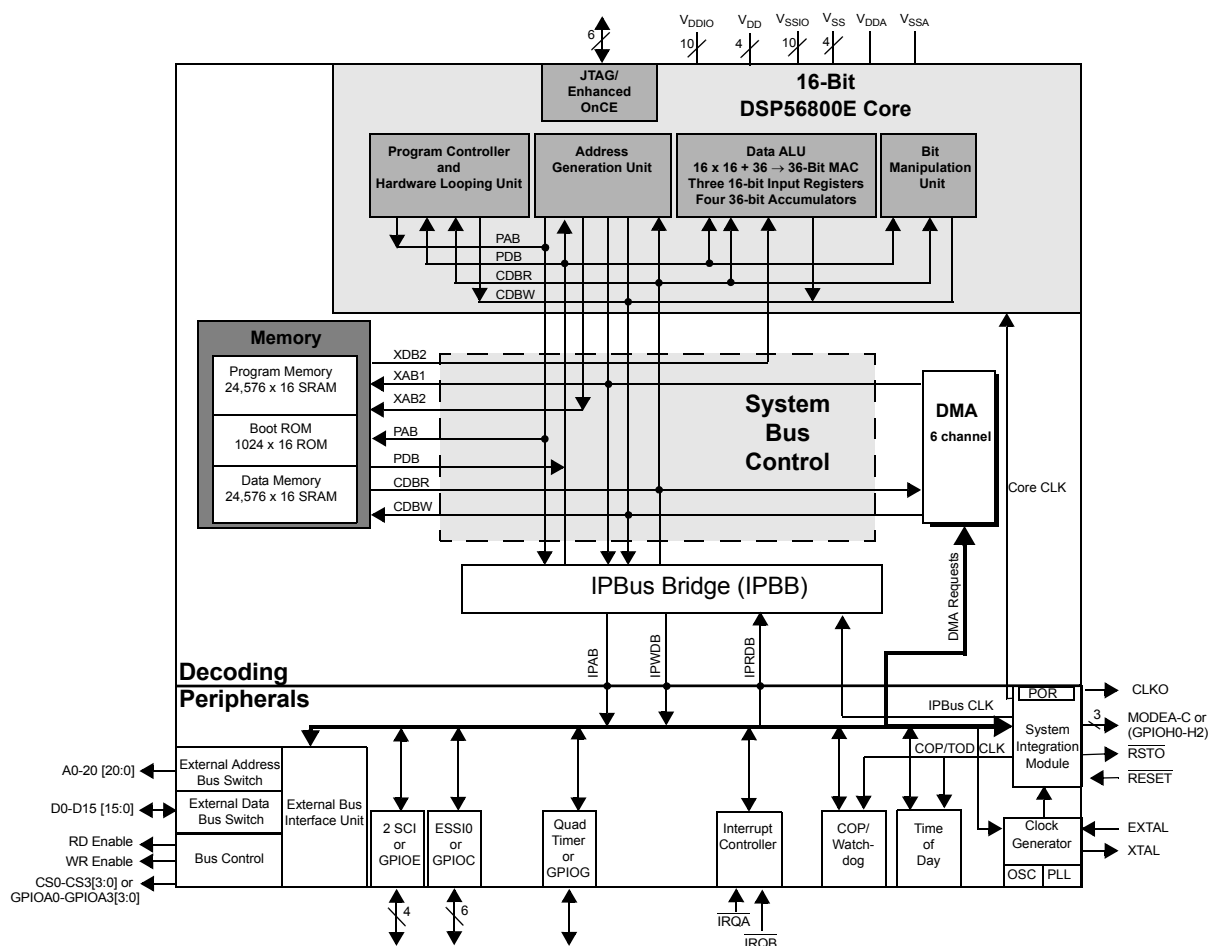
56855 Block Diagram
