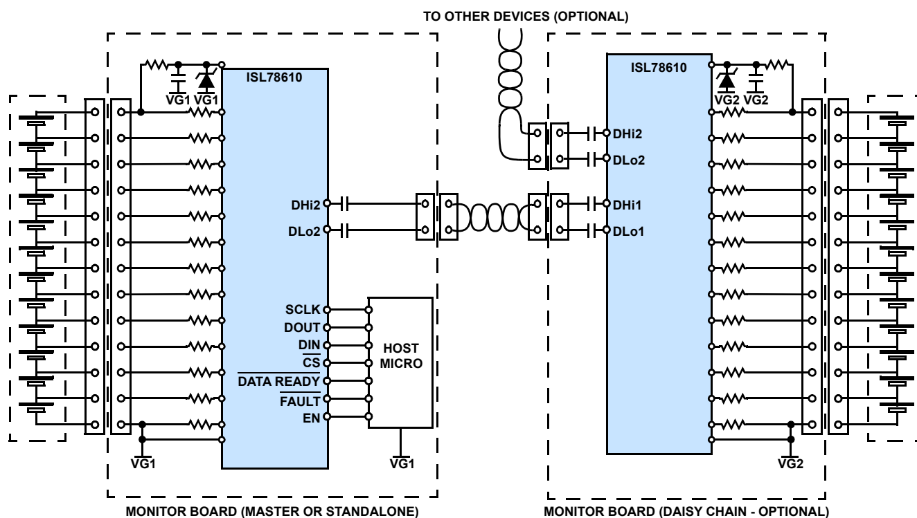
Figure 1. Typical Application
