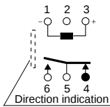
1-coil latching
