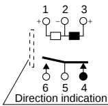
2-coil latching
