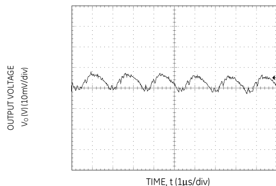
Figure 9. Typical output ripple and noise ( V_{IN} = 5V , I_o = I_{o,max} ).
