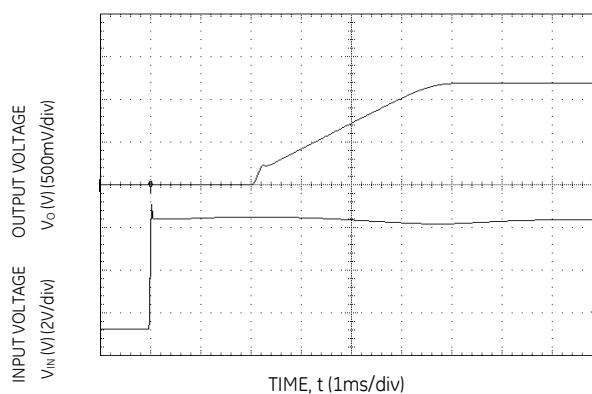
Figure 12. Typical Start-up Using Input Voltage ( V_{IN} = 5V , I_o = I_{o,max} ).
