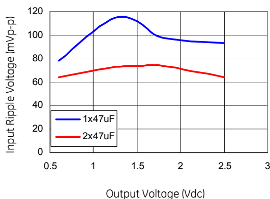
Figure 35. Input ripple voltage in mV, p-p for various output voltages with 1 \times 47\mu F or 2 \times 47\mu F ceramic capacitors at the input (12A load). Input voltage is 3.3V.
