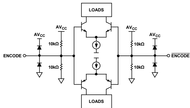
Figure 22. ENCODE/ENCODE-bar Inputs
