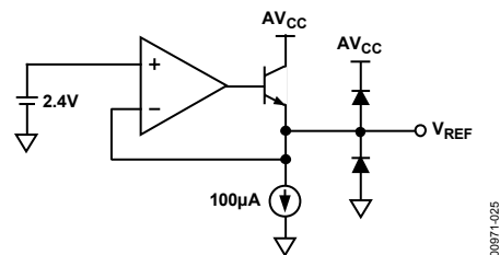
Figure 24. 2.4 V Reference
