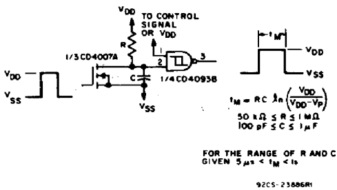
Fig. 17 - Monostable multivibrator.
