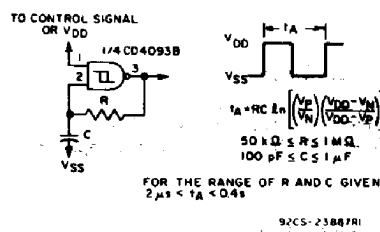
Fig. 18 - Astable multivibrator.
