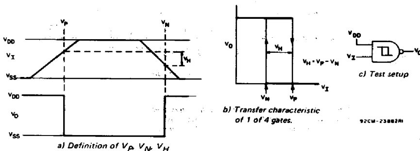
Fig. 2 - Hysteresis definition, characteristic, and test setup.
