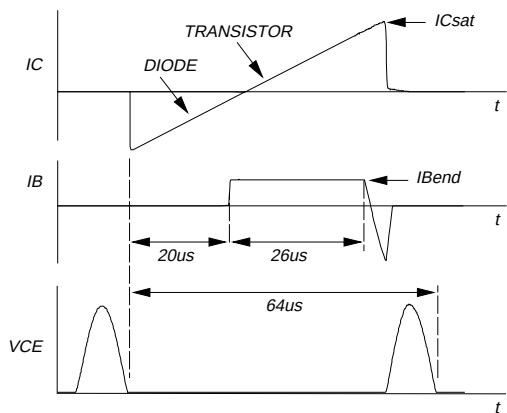
Fig.1. Switching times waveforms.
