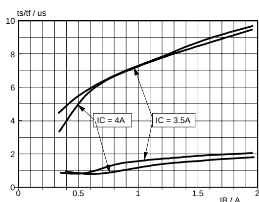
Fig.10. Limit storage and fall time. t_s = f(I_B) ; t_f = f(I_B) ; parameter I_C ; T_j = 85^\circ\text{C} ; f = 16\text{ kHz}
