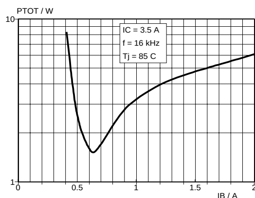
Fig.8. Limit P_{tot} ; T_j = 85^\circ\text{C} P_{tot} = f(I_{B(end)}) ; I_C = 3.5\text{ A} ; f = 16\text{ kHz}
