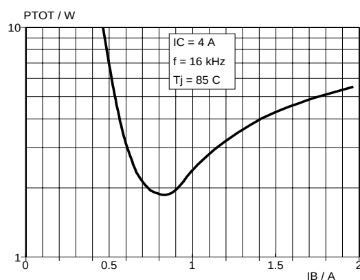
Fig.9. Limit P_{tot} ; T_j = 85^\circ\text{C} P_{tot} = f(I_{B(end)}) ; I_C = 4.0\text{ A} ; f = 16\text{ kHz}
