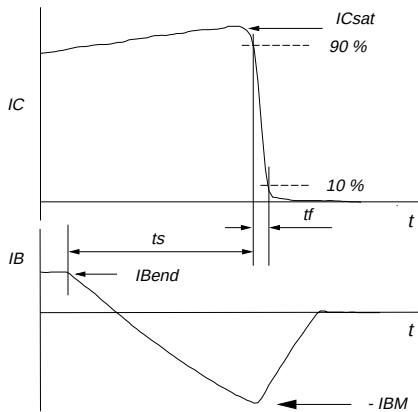
Fig.2. Switching times definitions.
