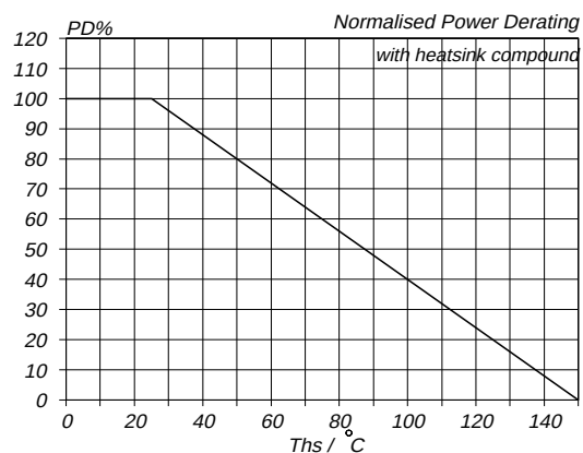
Fig.11. Normalised power dissipation. PD\% = 100 \cdot PD / PD_{25^\circ C} = f(T_{jhs})
