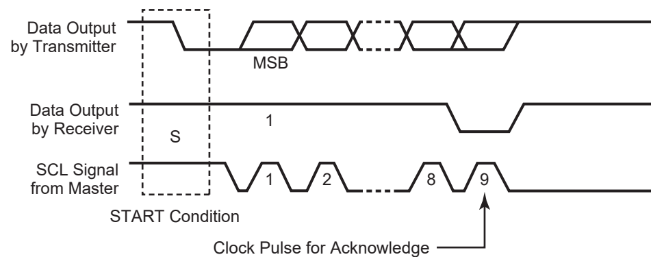
Figure 35. I²C Acknowledge
