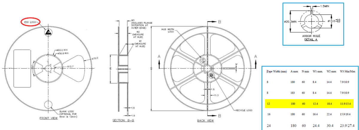
Figure 14. Reel information
