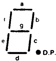
FIGURE 4. SEGMENT ASSIGNMENTS
