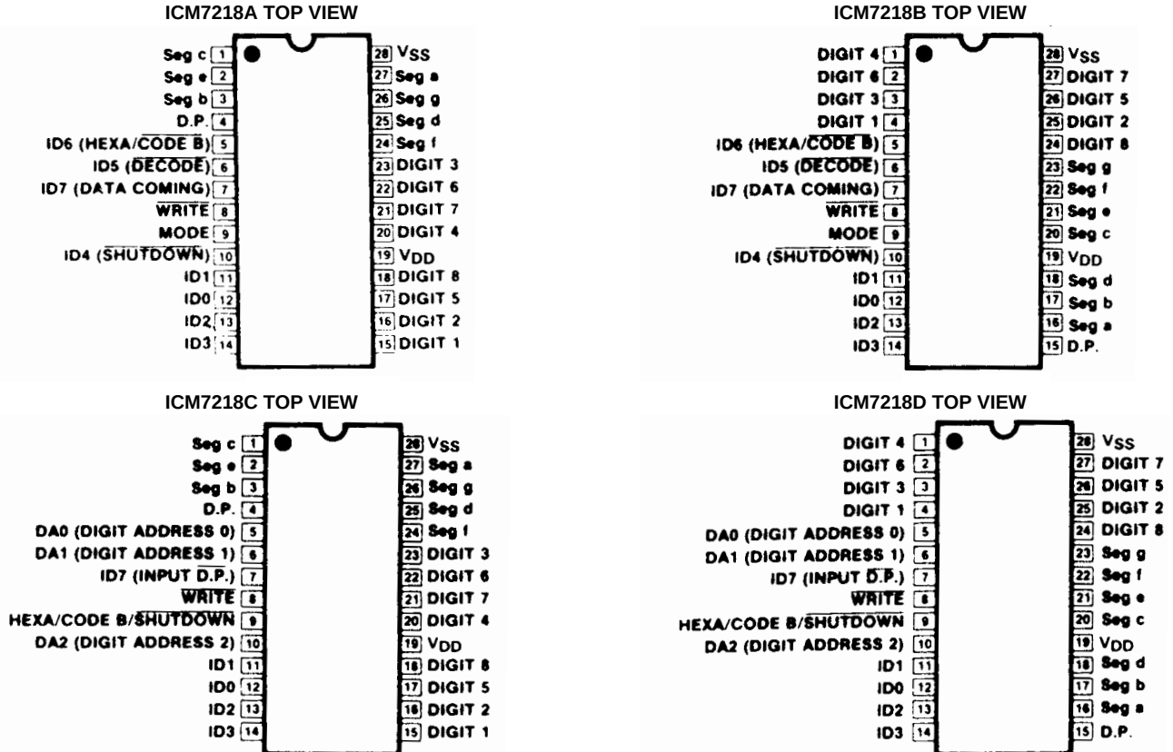
FIGURE 2. PIN CONFIGURATIONS
