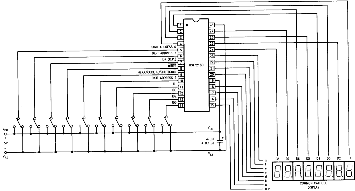
FIGURE 9. COMMON CATHODE DISPLAY FUNCTIONAL TEST CIRCUIT
