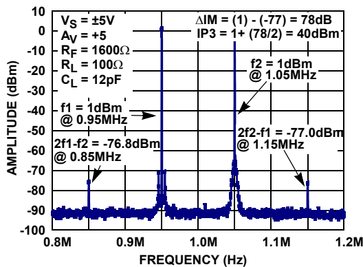
FIGURE 35. THIRD ORDER IMD INTERCEPT ( \text{IP}_3 )
