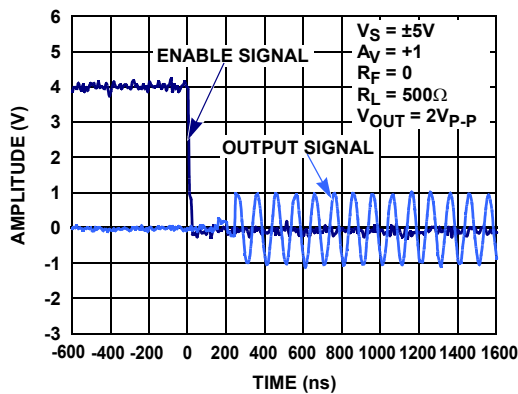
FIGURE 29. TURN-ON TIME
