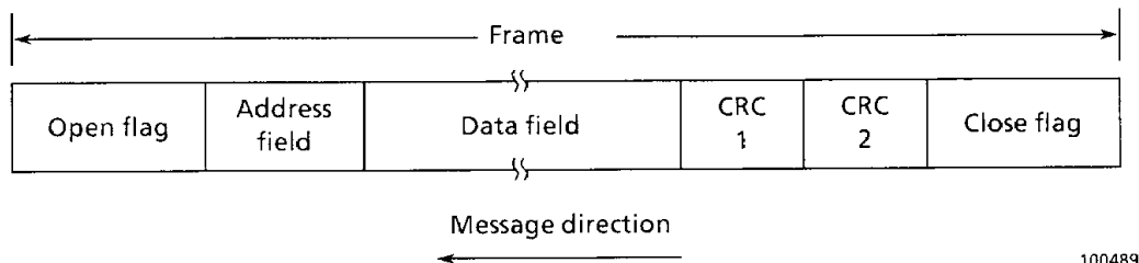
Figure 3.5 Data Format in SDLC Mode
