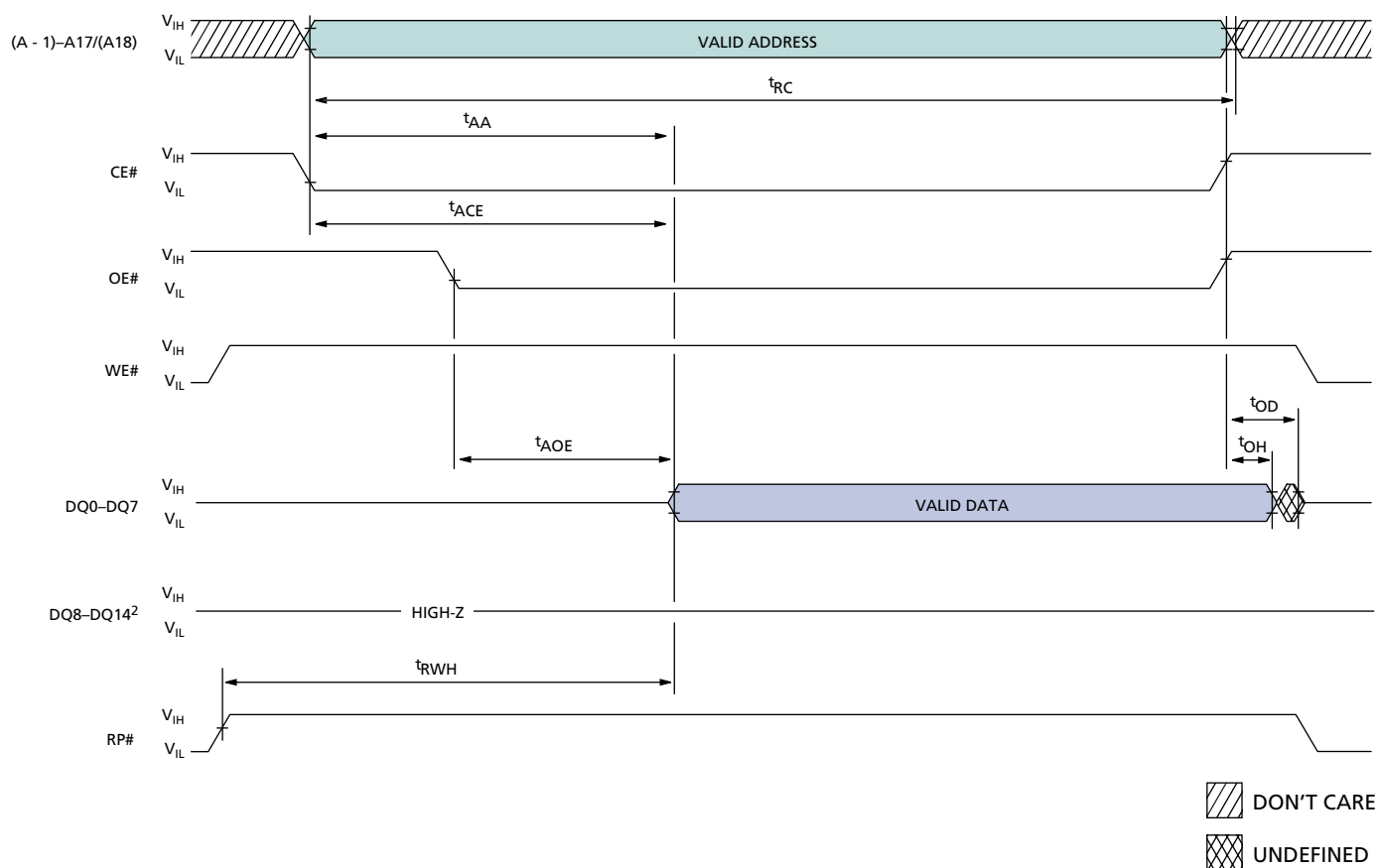
Figure 11: Byte-Wide READ Cycle 1
