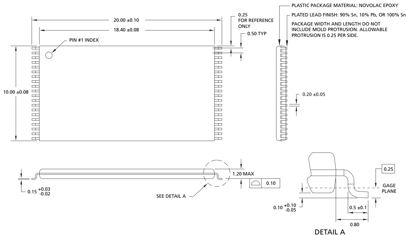
Figure 14: 40-Pin Plastic TSOP I (10mm x 20mm)
