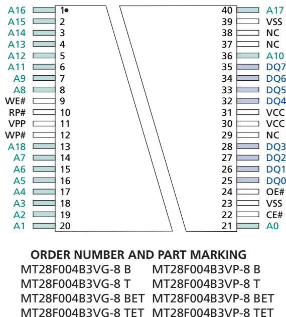
40-Pin TSOP Type I
