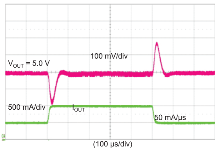
Transient Response 0.5 to 1 A Load Step at V_{IN} = 5\text{ V} for 5 V_{OUT} , 2 MHz design example
