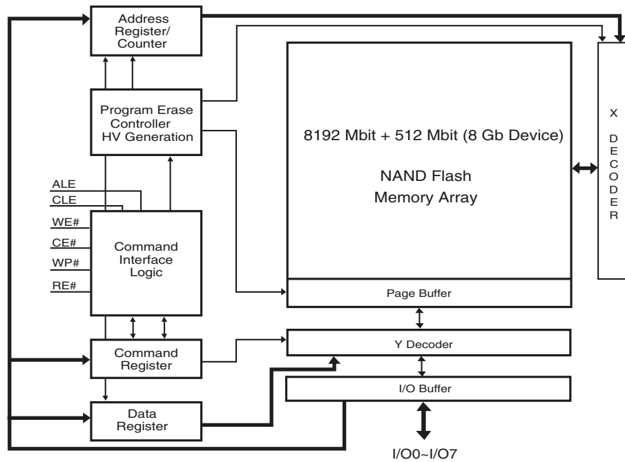
Figure 4.1 Functional Block Diagram — 8 Gb
