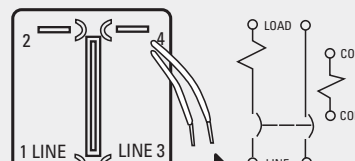
Two Pole (1 pole relay)
