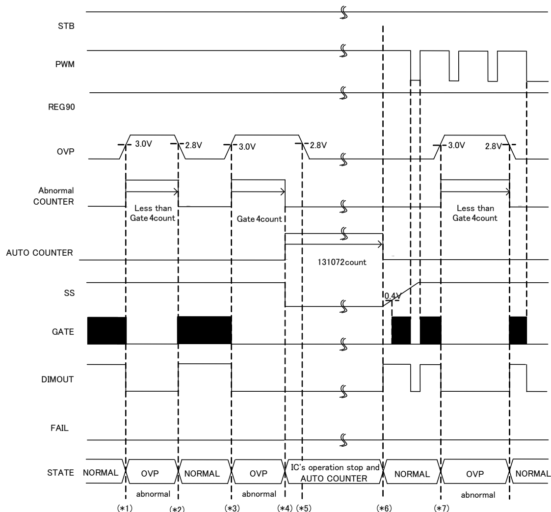
Figure 34. OVP Detection
