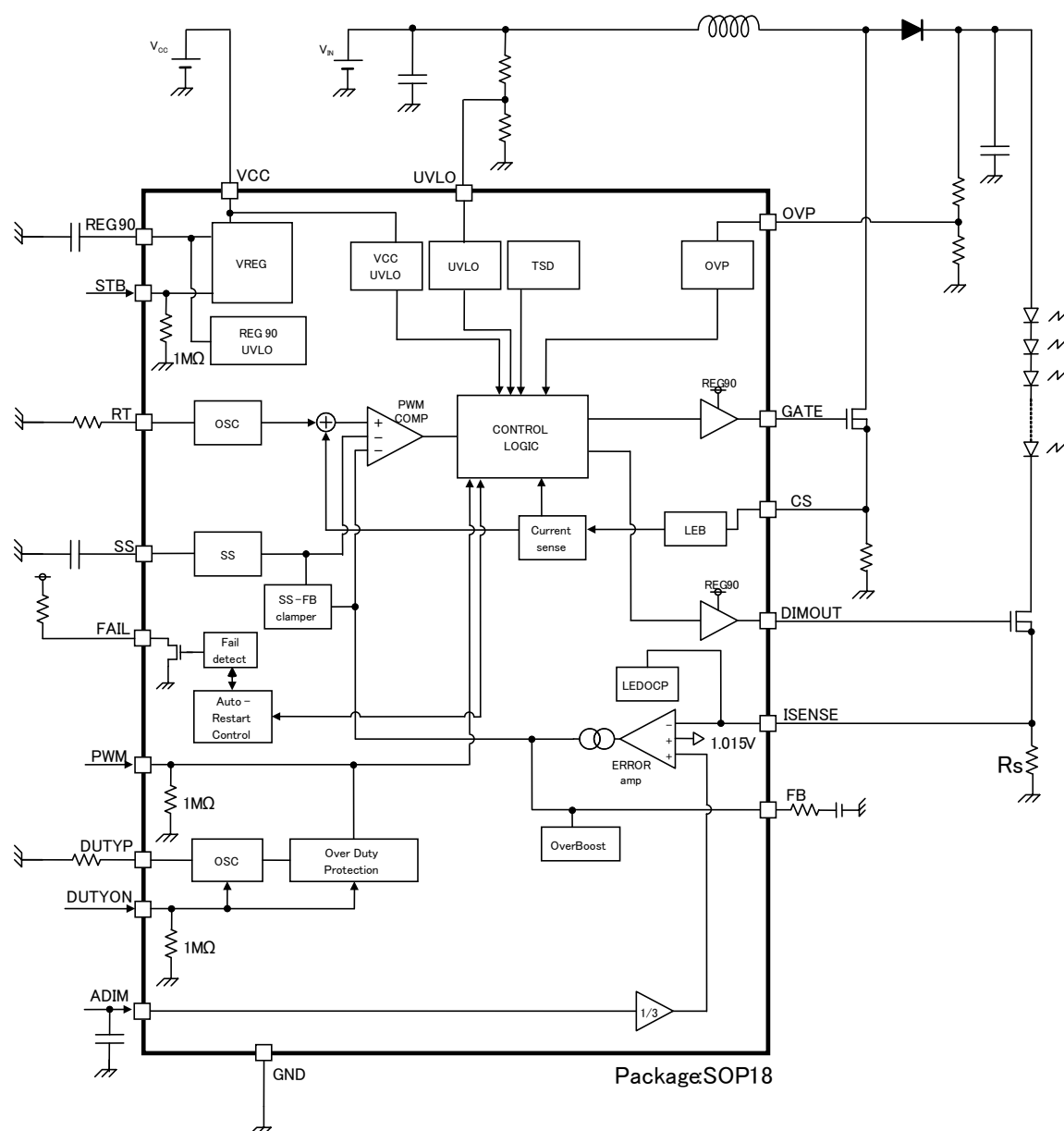
Figure 4. Block Diagram
