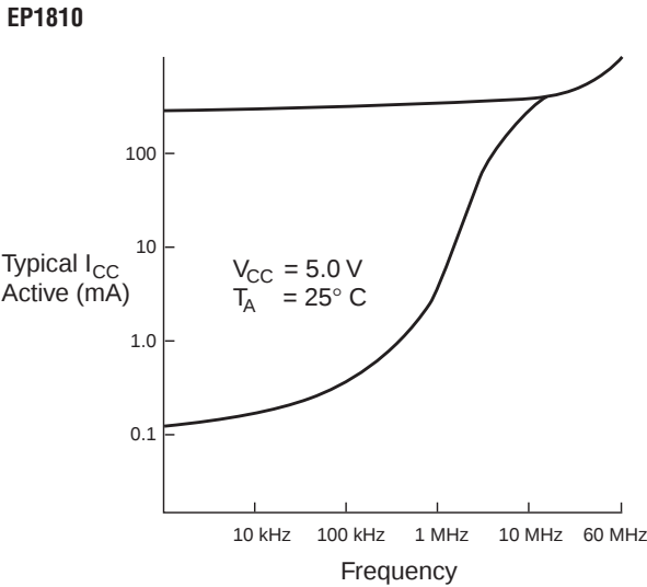
Figure 17. I_{CC} vs. Frequency of EP1810 Devices
