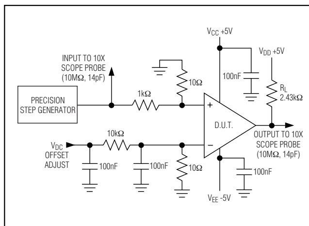
Figure 5. Response-Time Setup
