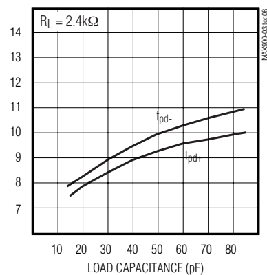
RESPONSE TIME vs. LOAD CAPACITANCE (5mV OVERDRIVE)
