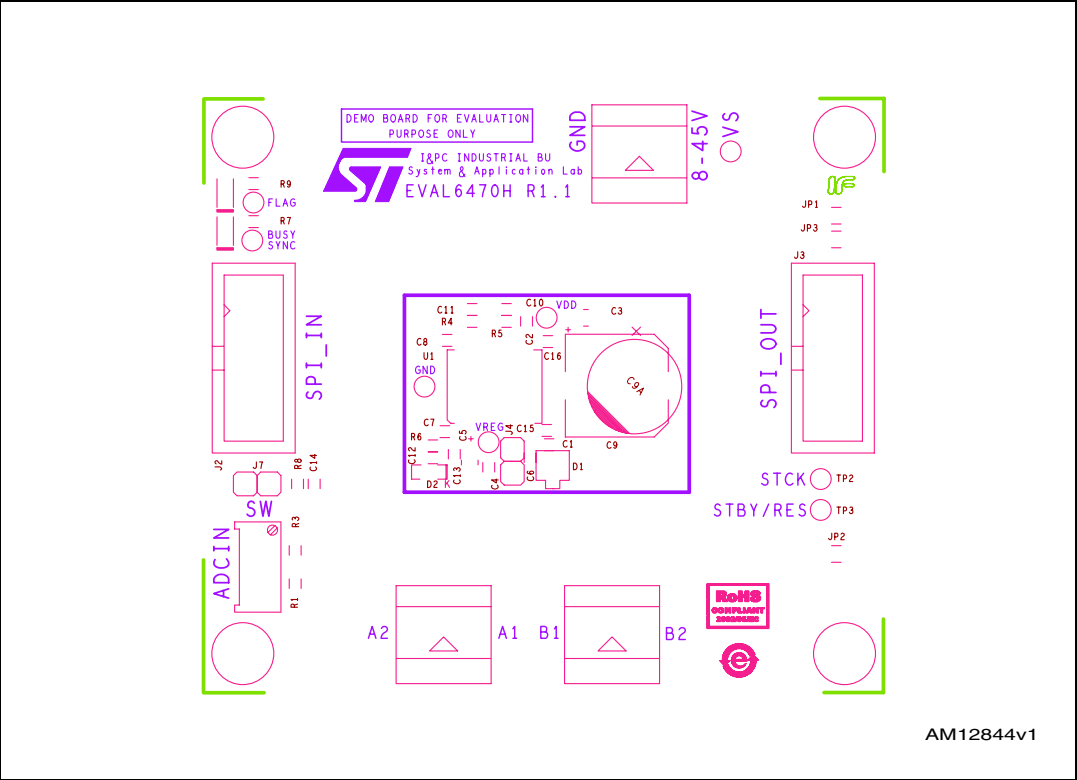
Figure 3. EVAL6470H - layout (silk screen)
