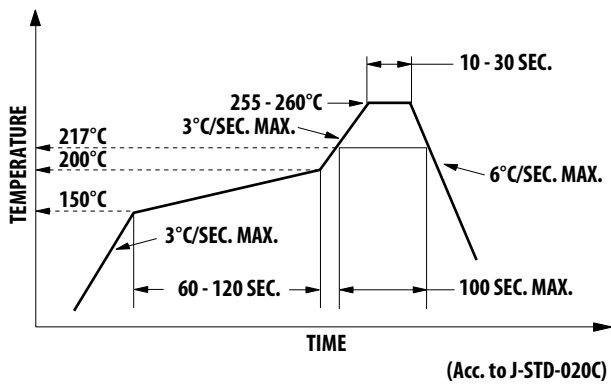
Figure 8. Recommended Reflow Soldering. (Acc. to J-STD-020C)
