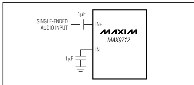
Figure 6. Single-Ended Input
